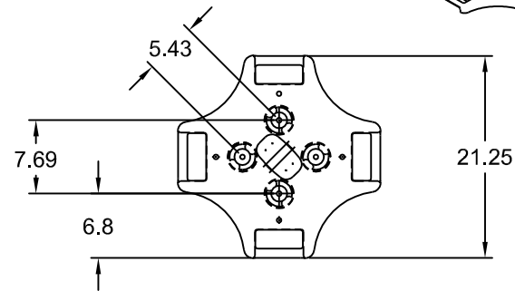
BASE DETAIL
